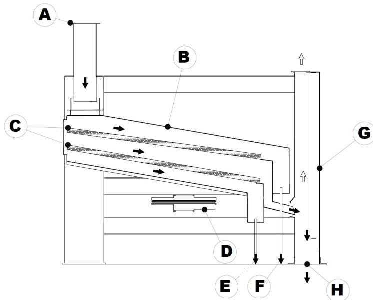
Sectional Informational View on Single Deck Cleaner
