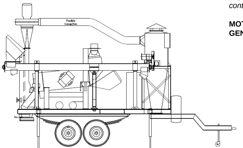
Side elevation - Transport position
