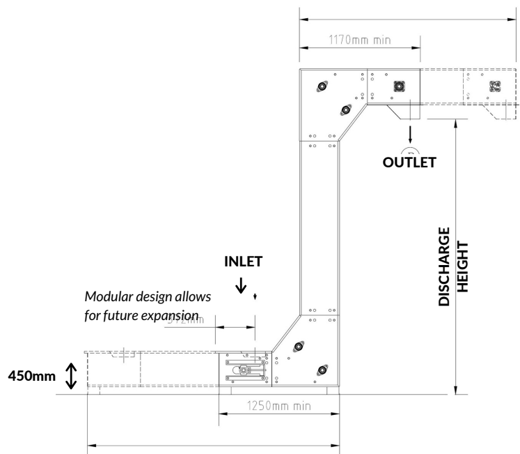
Swing Tray Bucket Elevator side view
